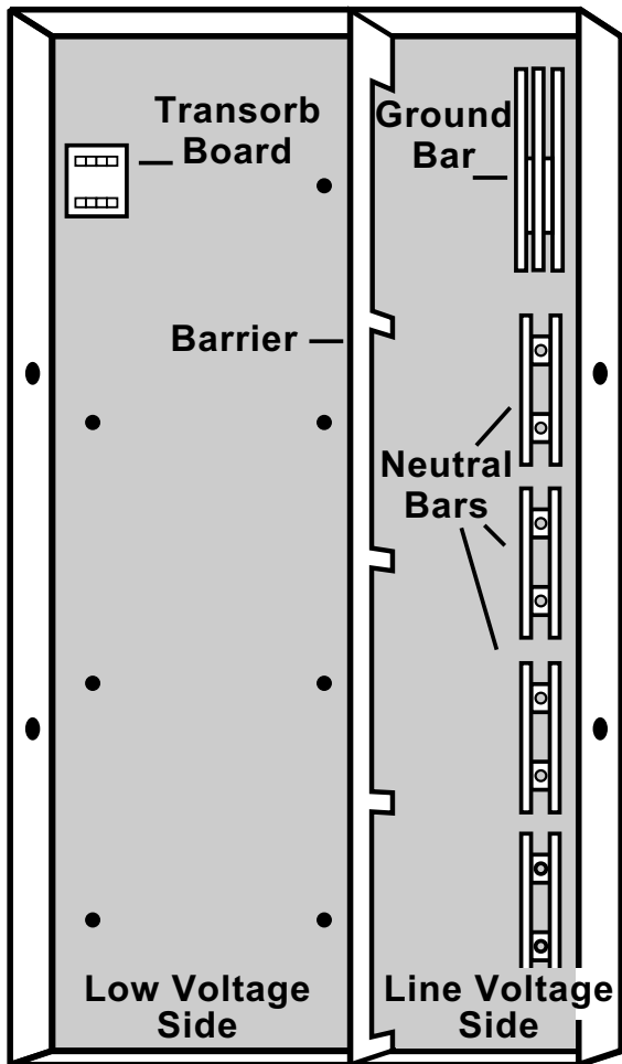
Four Module Enclosure
